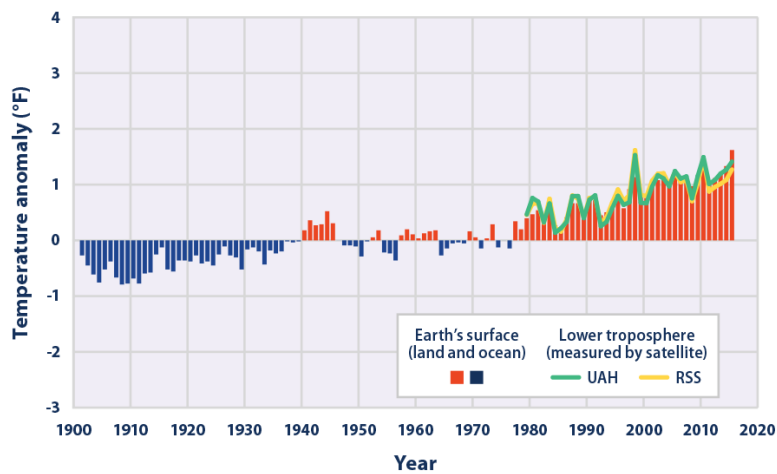
Temperatures Worldwide, 1901–2015
